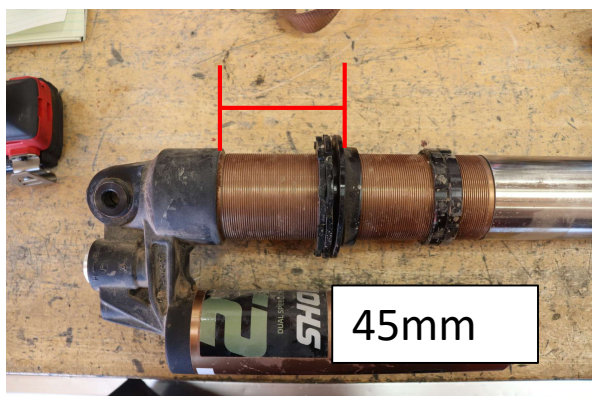
Step 11. Set pre-load spring seat to 45mm (1 3/4in.) from bottom of seat to bottom of reservoir bridge.
