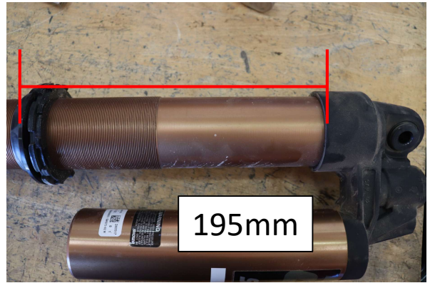
Step 10. Set pre-load to 195mm (7 11/16 in.) from bottom of spring seat to bottom of furthest point on reservoir bridge.
